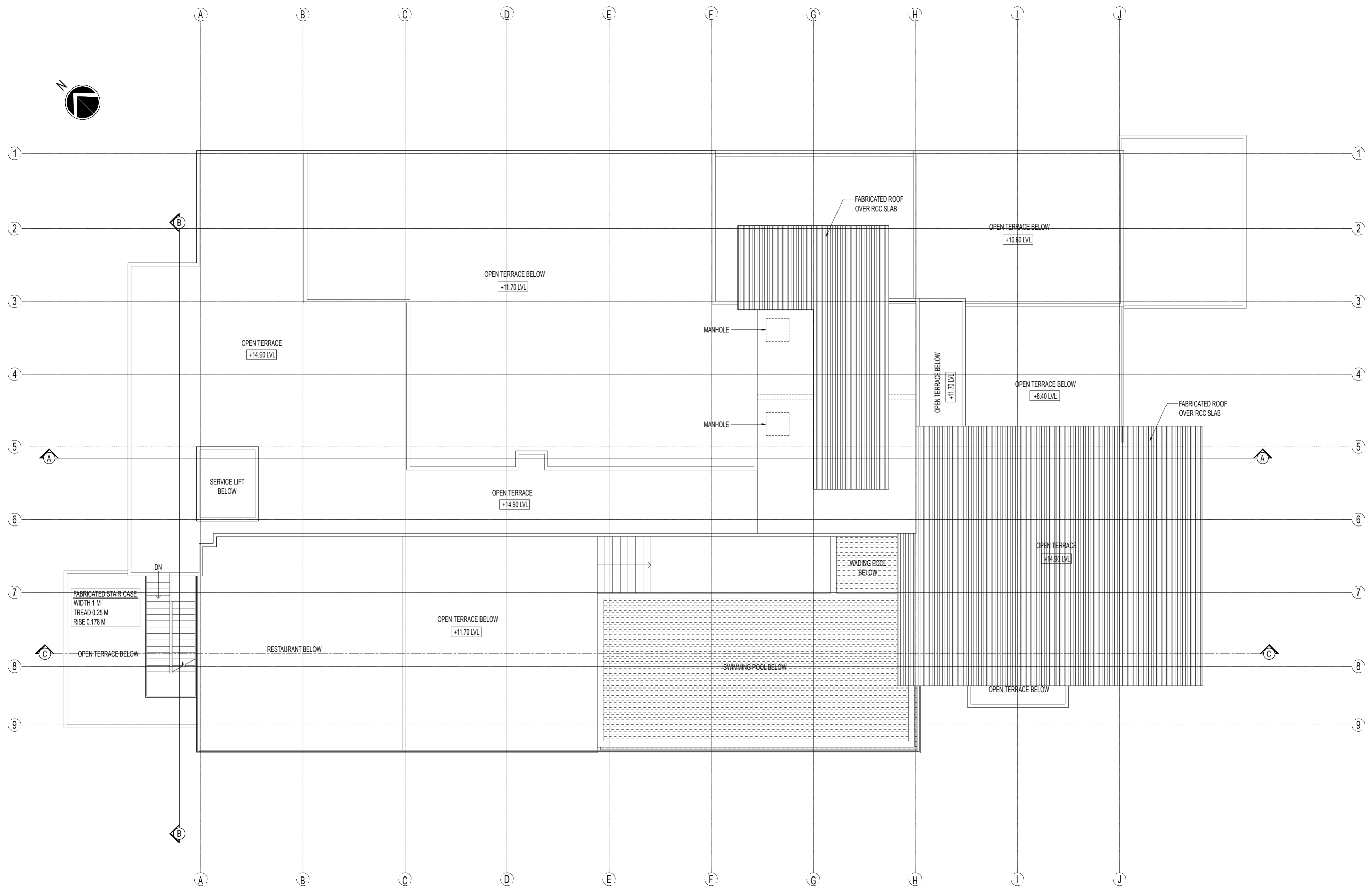
TERRACE PLAN AT ROOF LEVEL SCALE 1:100
