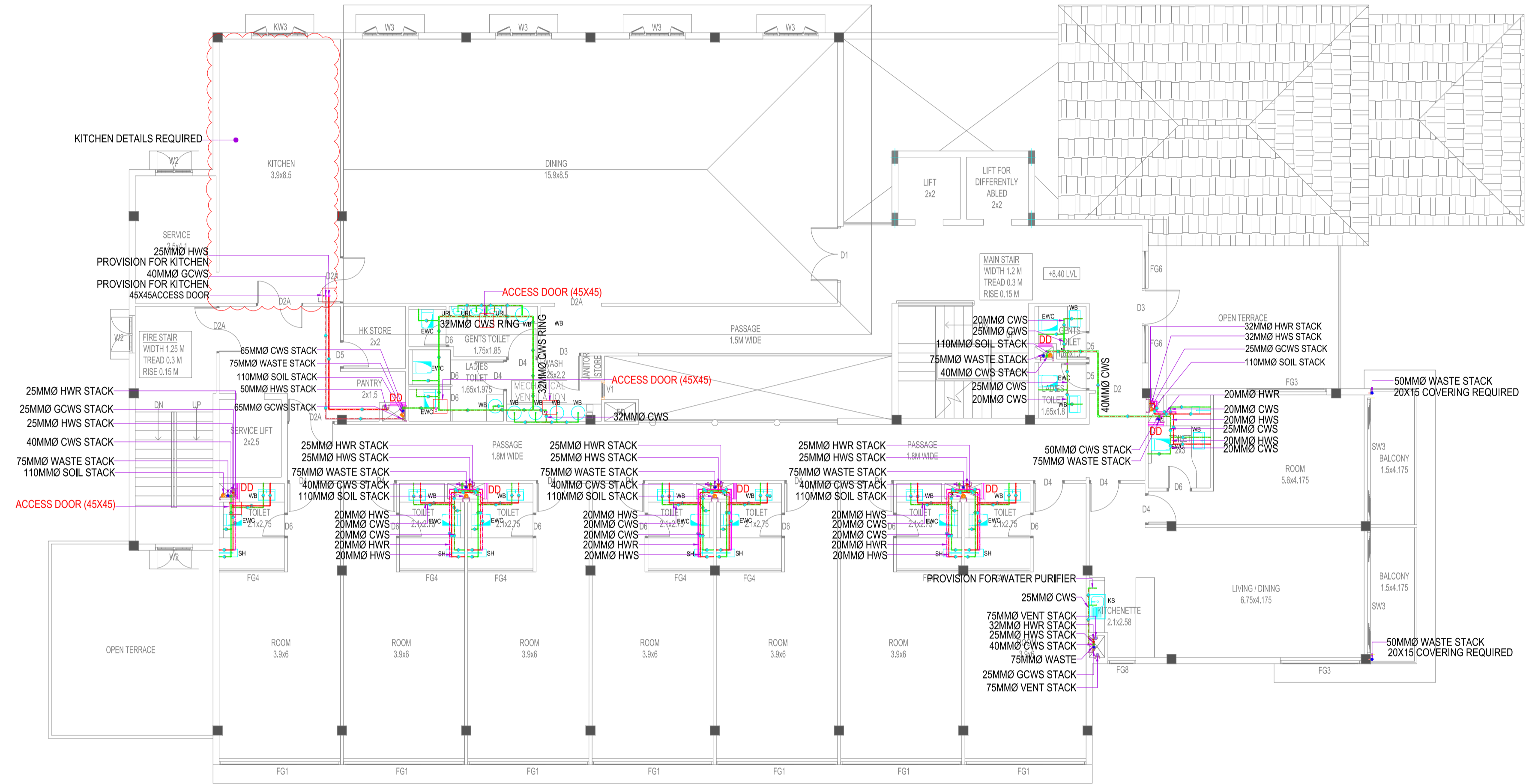
SECOND FLOOR SCALE 1:100
